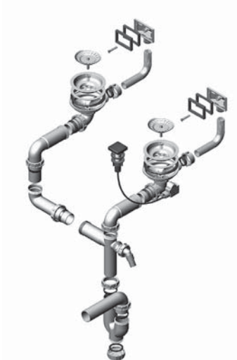
Waste kit 2XQMH 114 - PP - 114 - PP POP - UP
