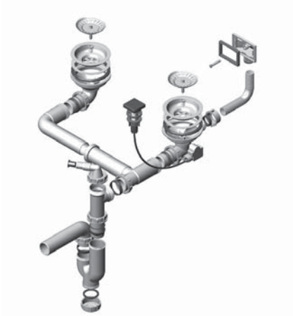
Waste kit 2XQM 114 - PP - 114 POP- UP
