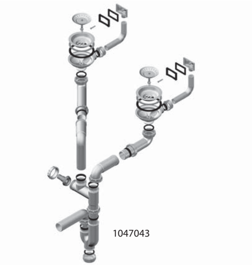
Waste kit 2XSPH 114 - PP - 114 - PP
