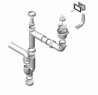
Waste kit 1XSP 70 - PP
