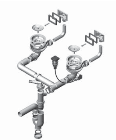
Waste kit 2XQM 114 - PP - 114 - PP POP - UP
