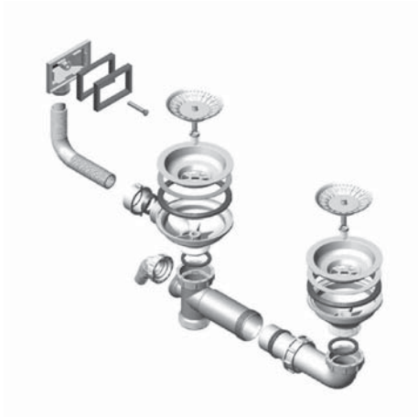
Waste connection 114-PP-114
