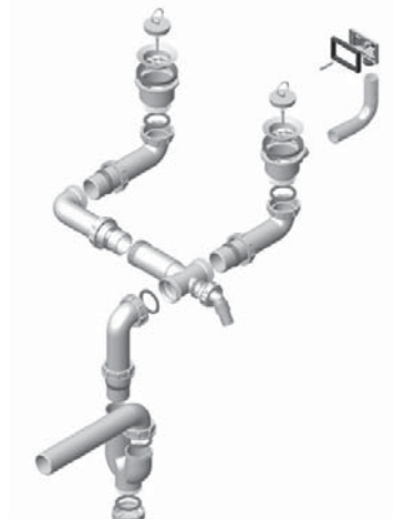
Waste kit 2XSP 70 - PP - 70
