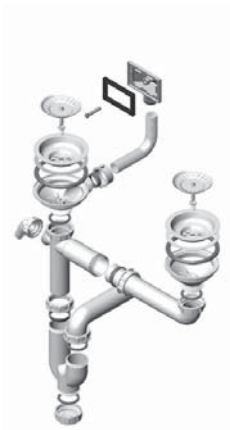
Waste kit 2XSL 114 - PP - 114
